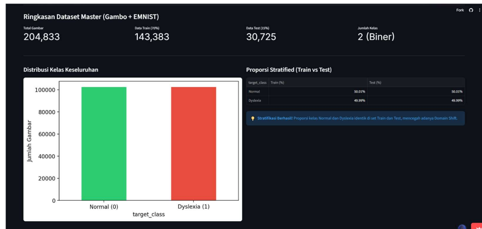
Gambar 16. Dashboard Streamlit
